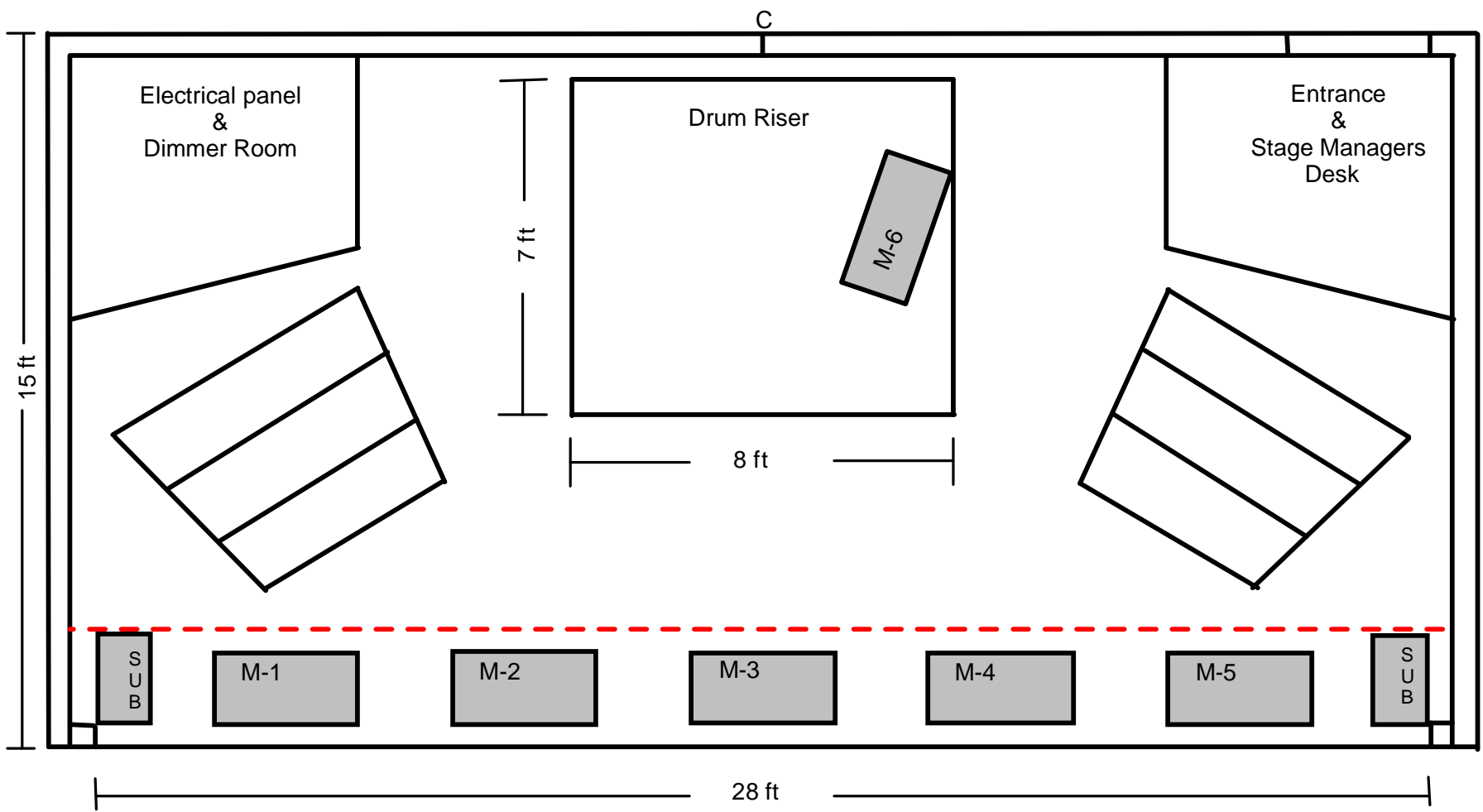
Grassy Plains Summer Festival 2015 Outdoor Stage Ground Plan (with choral risers)
